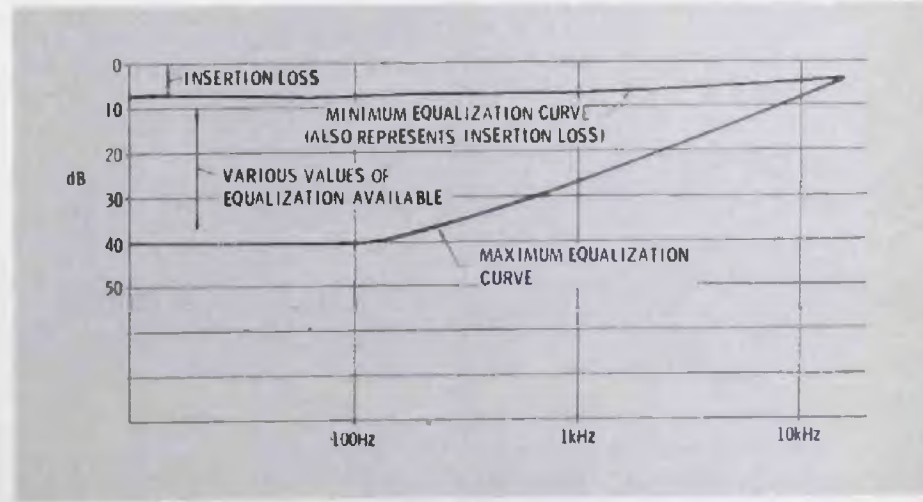
Fig. 5 Typical equalization curve of a small commercial equalizer. There is an insertion loss of about 7 dB. About 35 dB equalization is possible at the low end.
