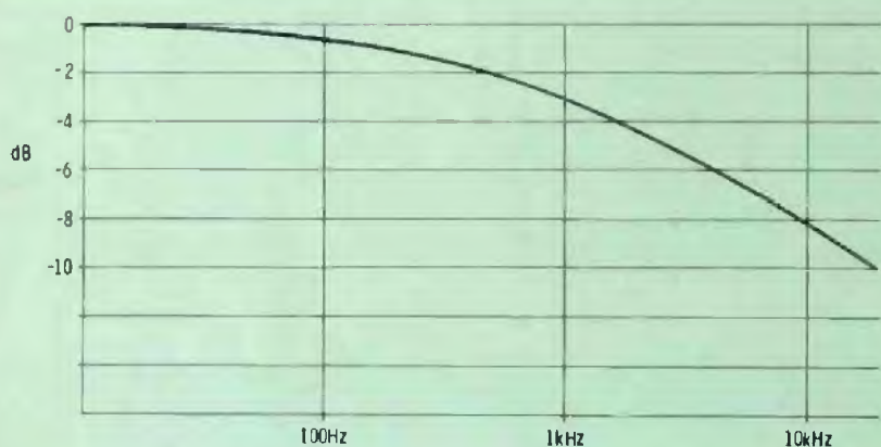
Fig. 3 Typical response of one mile of telco line.
