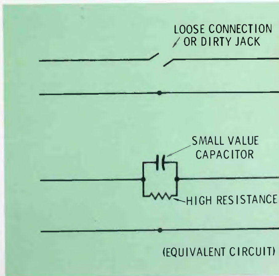
Fig. 2 A dirty or loose connection can have the effect of inserting a high resistance and small value capacity in series with the line. This will affect the low frequency response.
