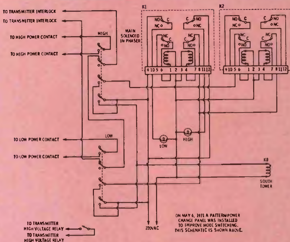
Fig. 2 Schematic of the KXRO changeover panel.
